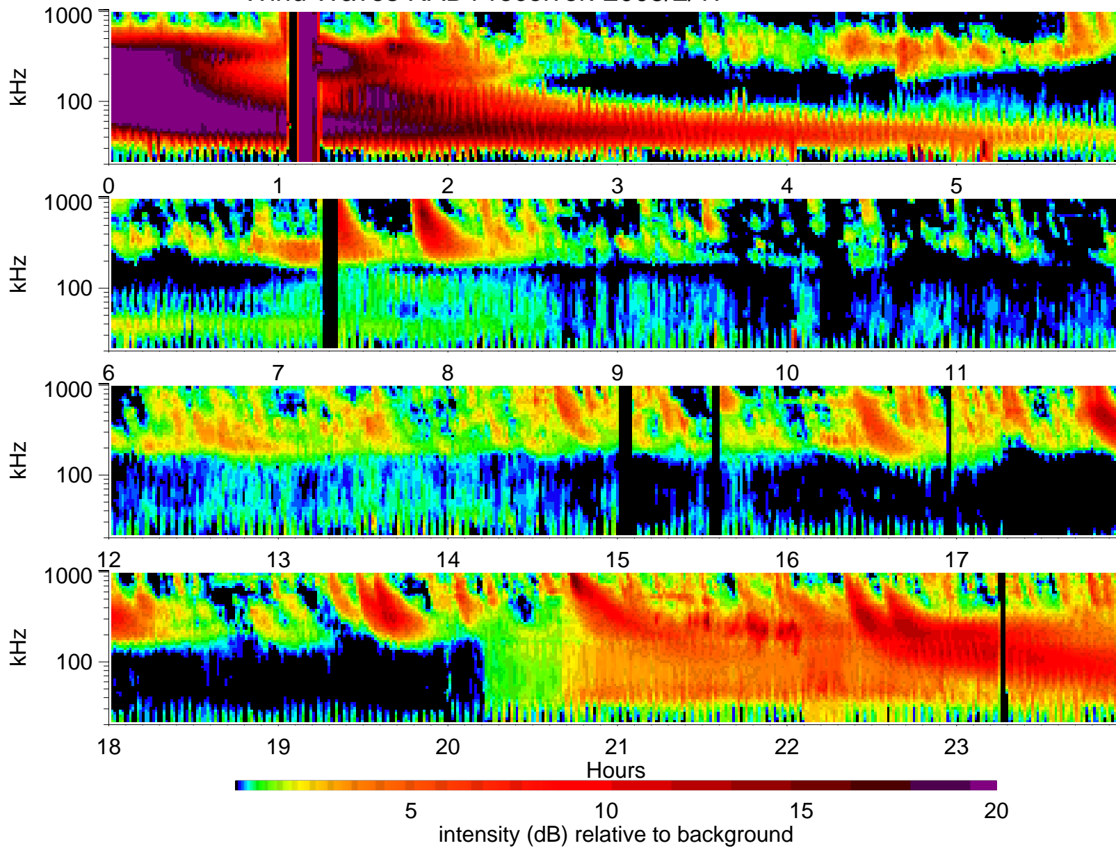
Wind Waves RAD1 receiver: 2005/2/17
