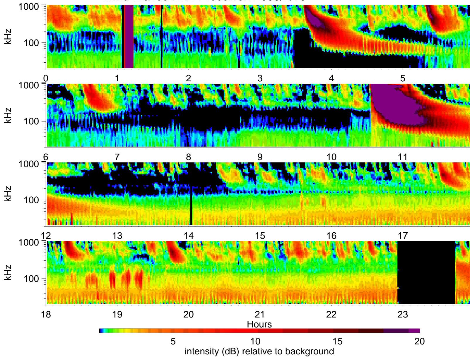
Wind Waves RAD1 receiver: 2005/2/13
