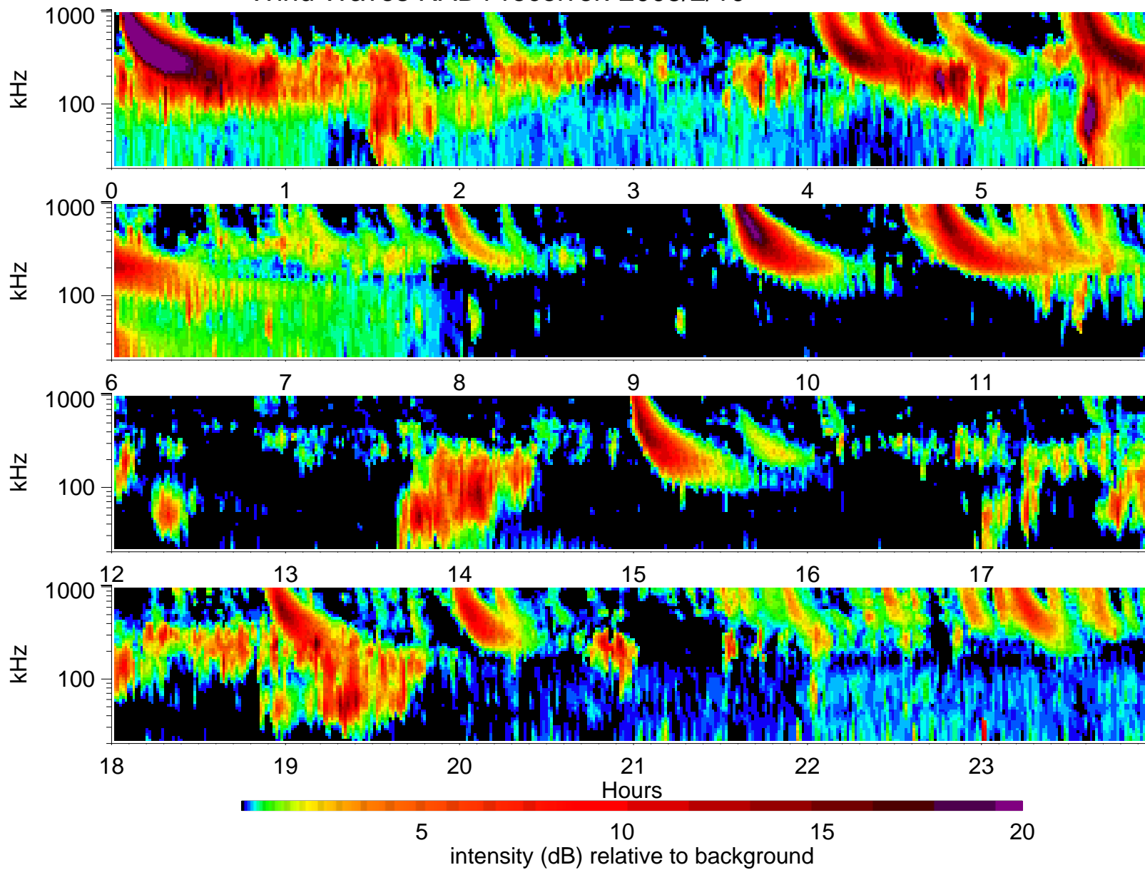
Wind Waves RAD1 receiver: 2005/2/10
