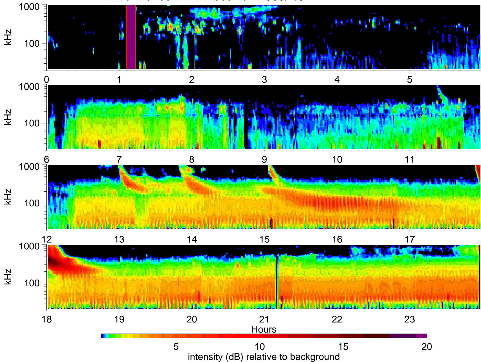
Wind Waves RAD1 receiver: 2005/2/5
