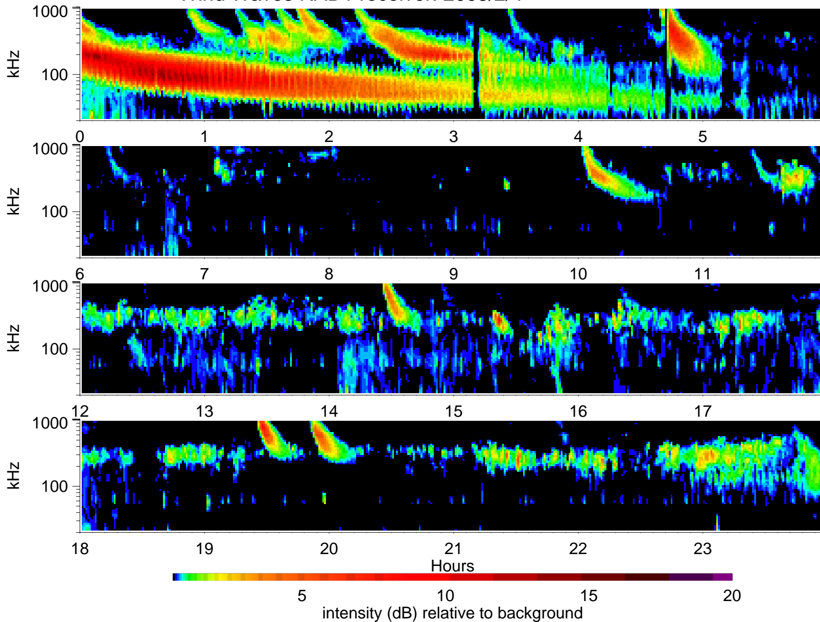
Wind Waves RAD1 receiver: 2005/2/4
