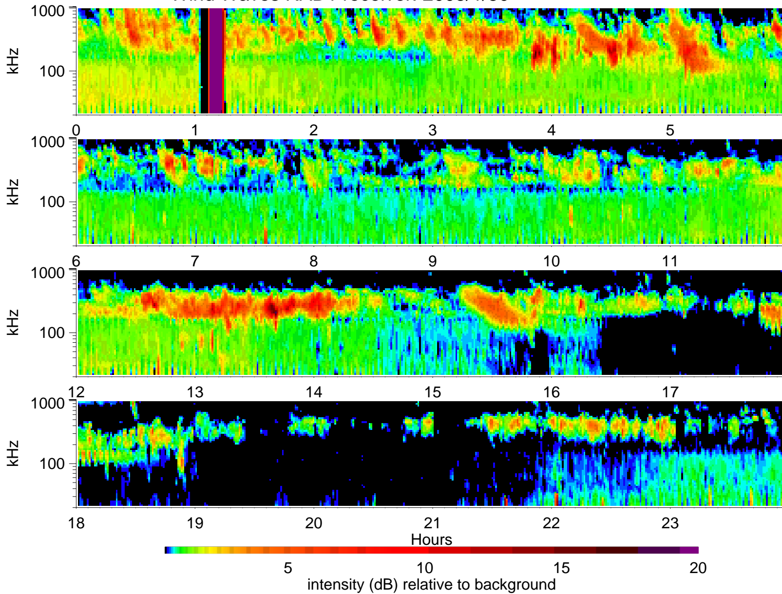
Wind Waves RAD1 receiver: 2005/1/30
