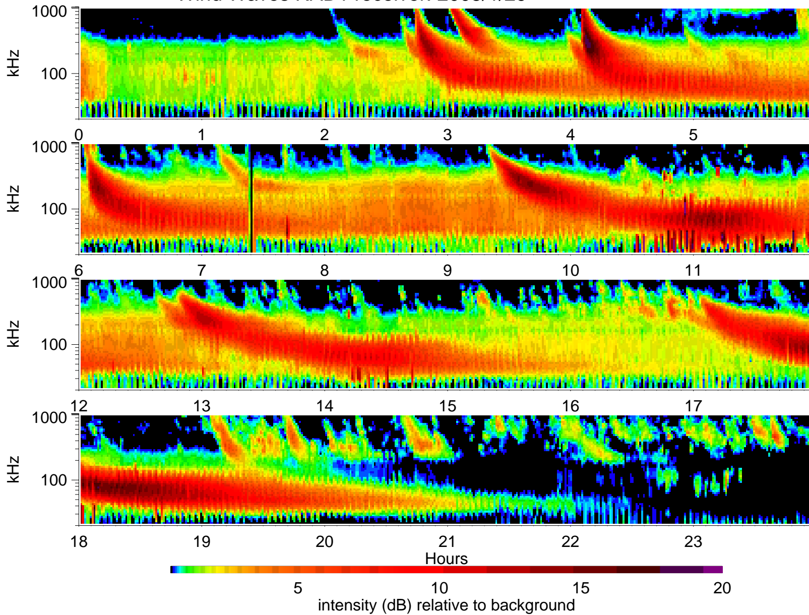
Wind Waves RAD1 receiver: 2005/1/29
