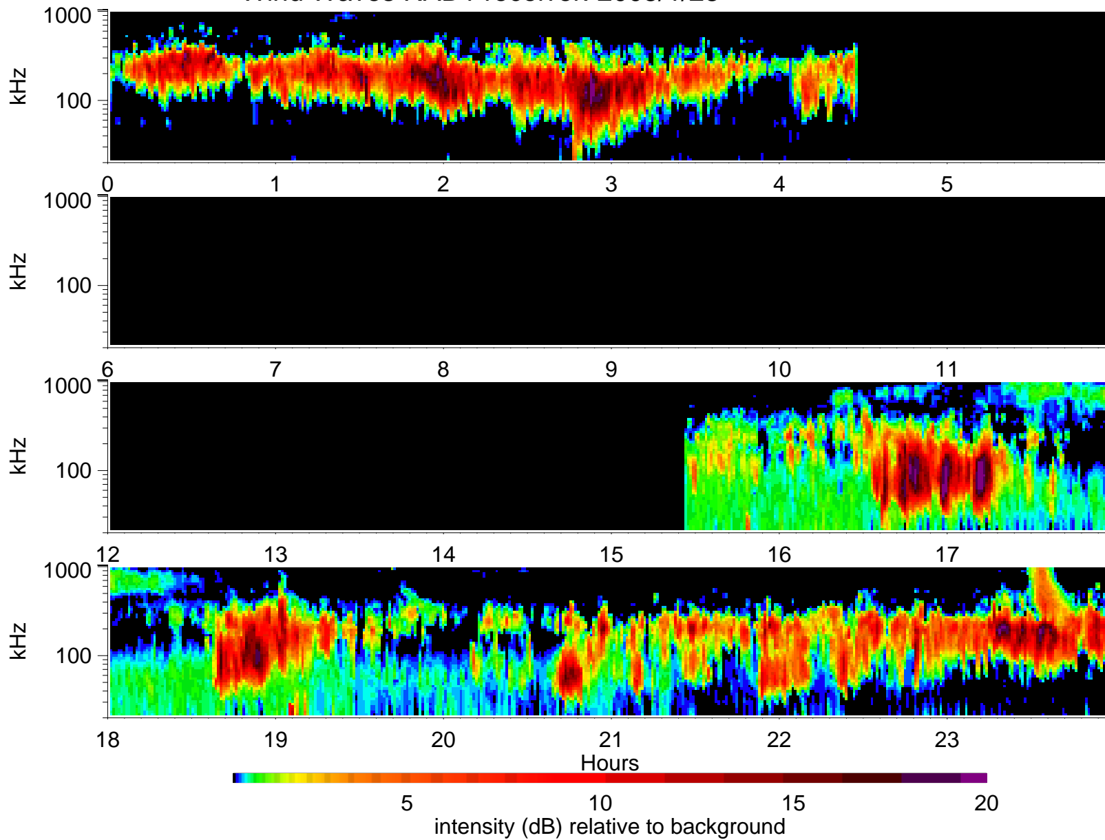
Wind Waves RAD1 receiver: 2005/1/23
