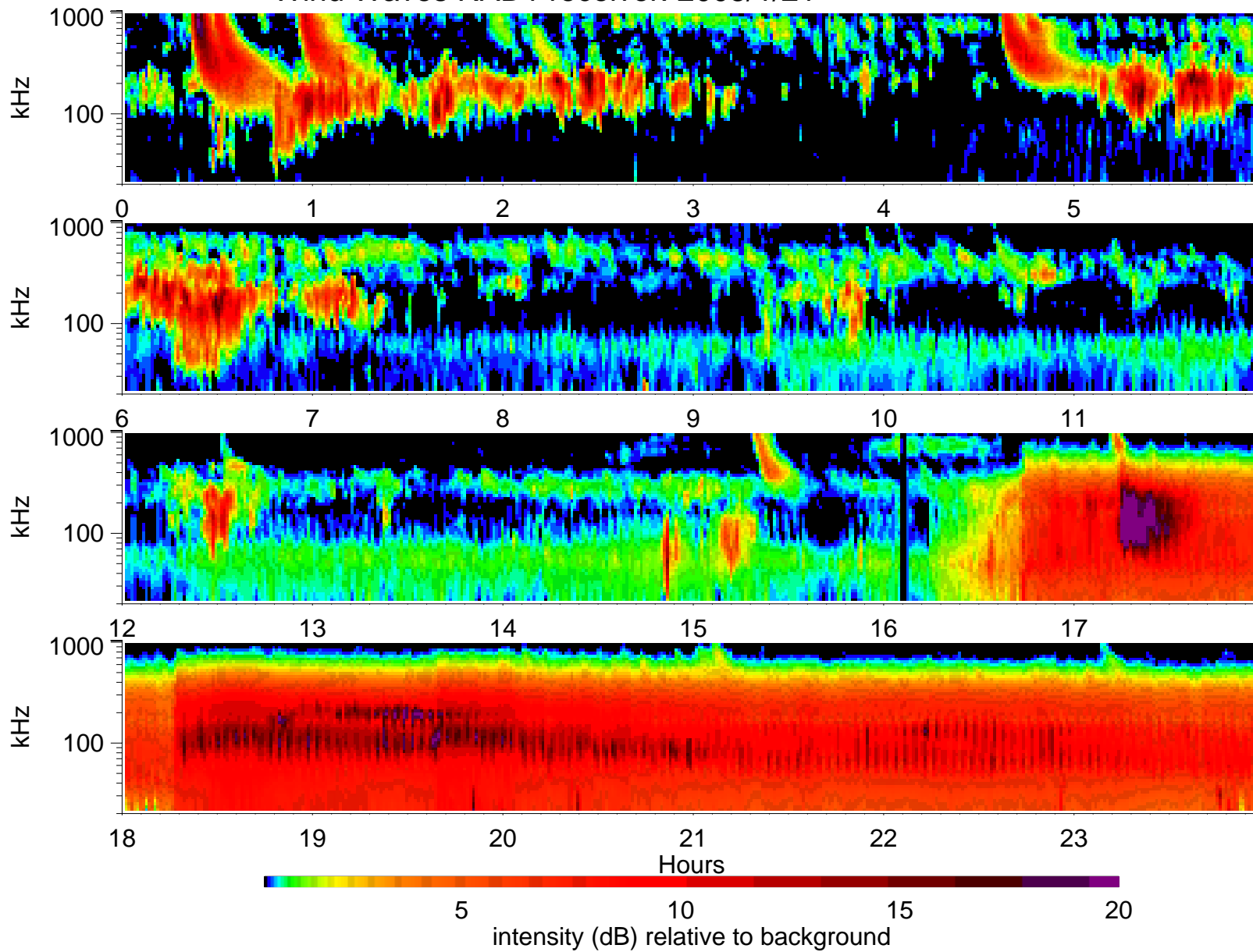
Wind Waves RAD1 receiver: 2005/1/21
