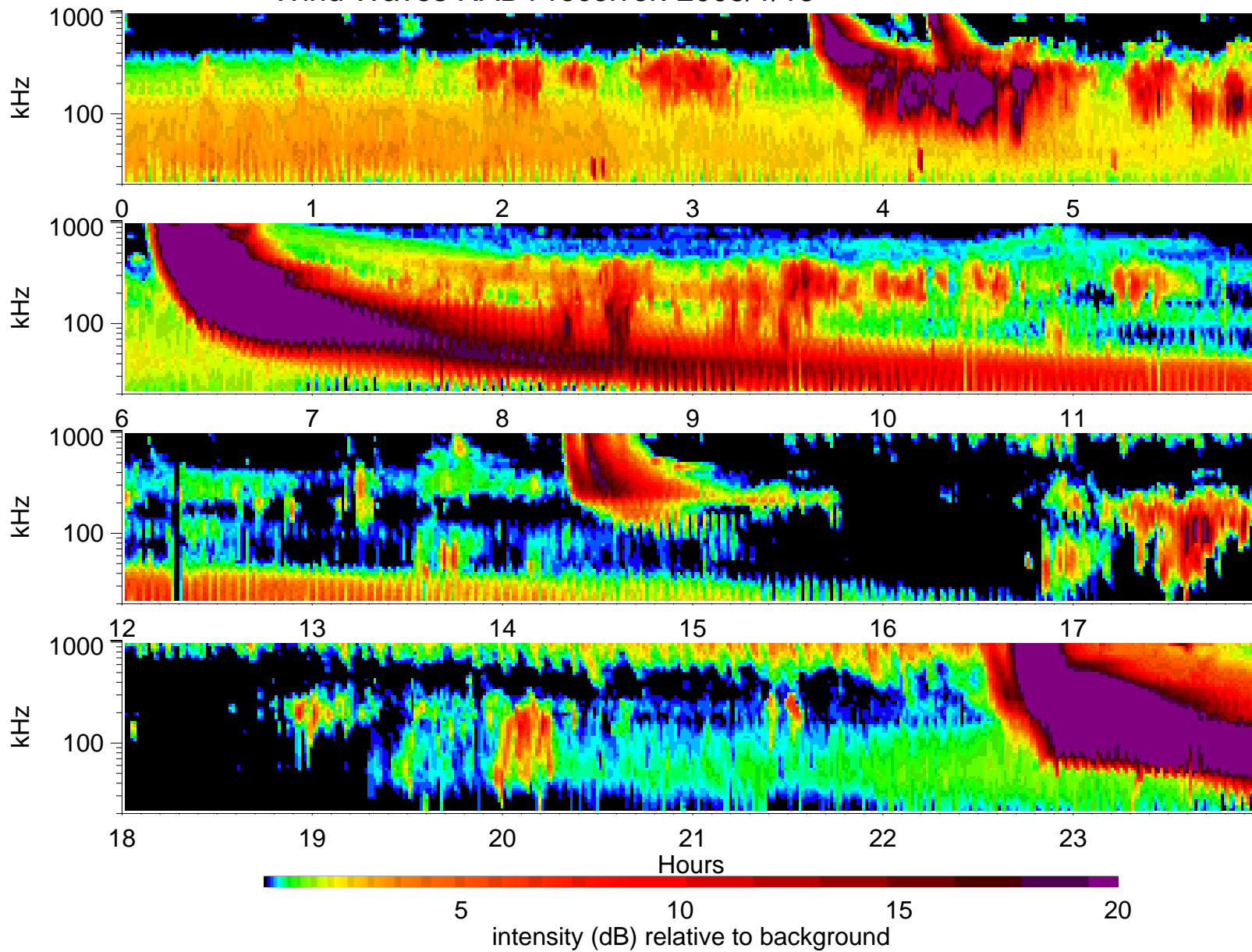
Wind Waves RAD1 receiver: 2005/1/15
