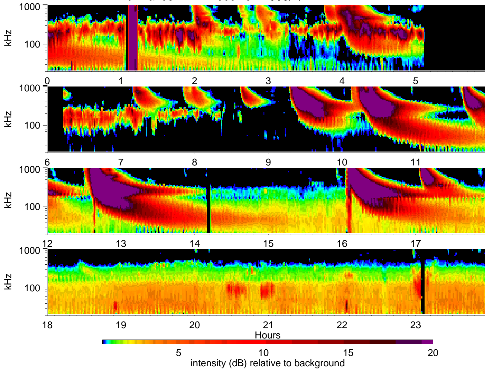
Wind Waves RAD1 receiver: 2005/1/14
