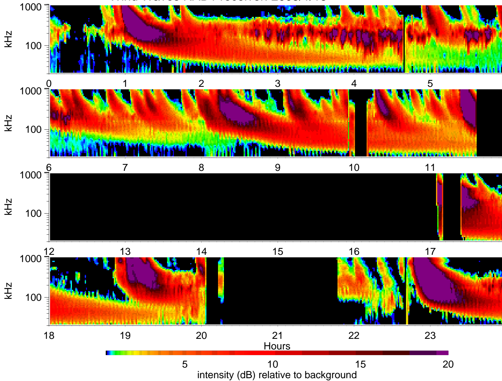
Wind Waves RAD1 receiver: 2005/1/13
