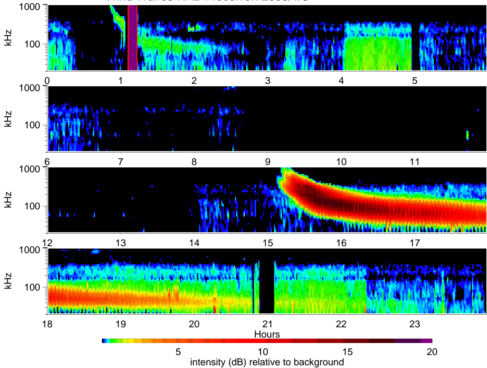
Wind Waves RAD1 receiver: 2005/1/6
