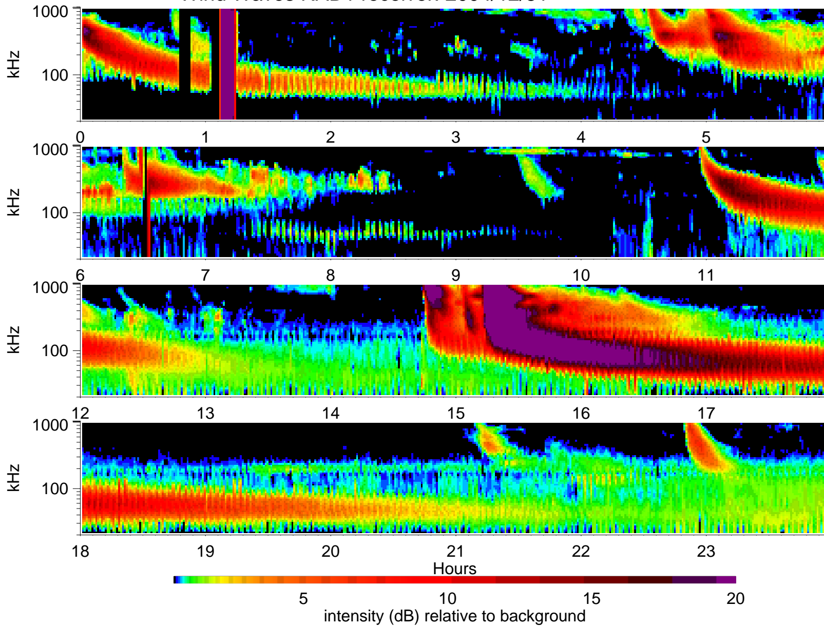
Wind Waves RAD1 receiver: 2004/12/31
