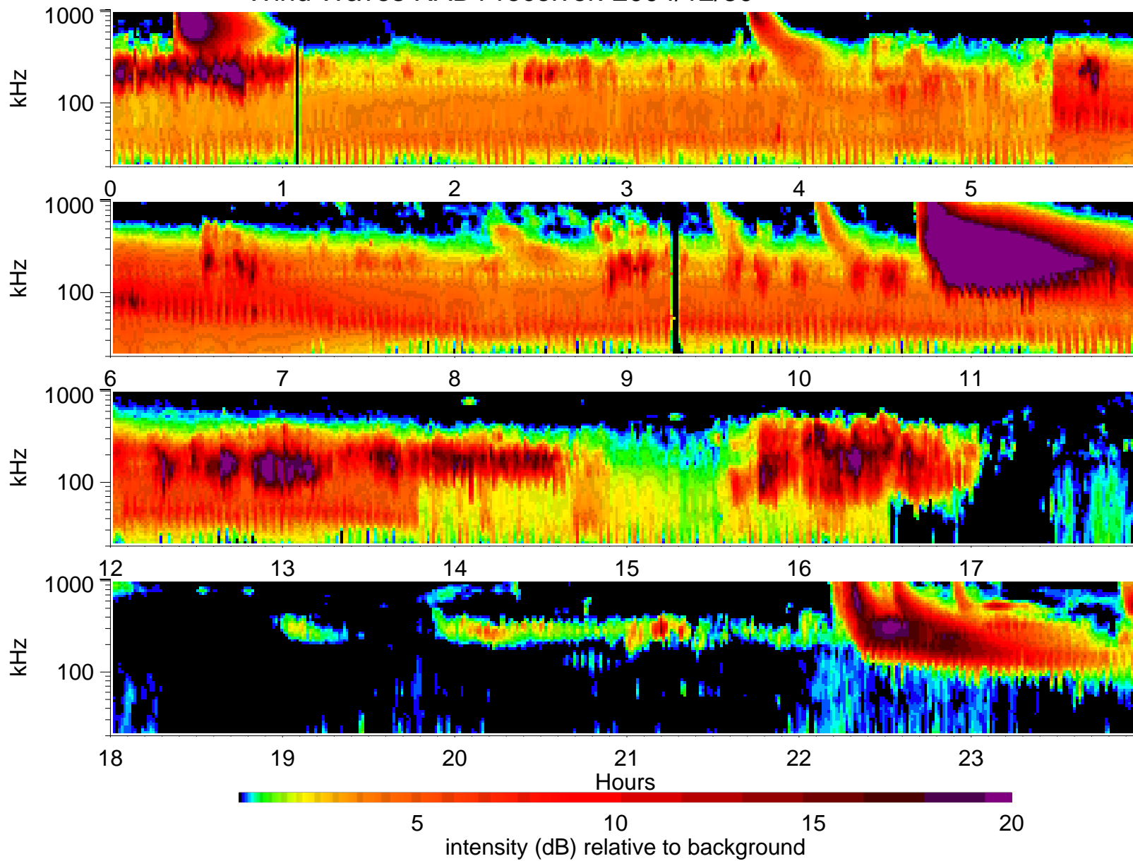
Wind Waves RAD1 receiver: 2004/12/30
