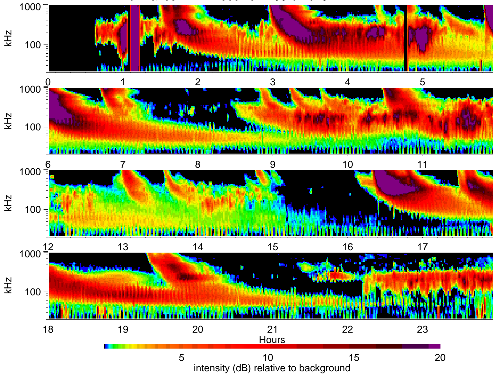
Wind Waves RAD1 receiver: 2004/12/29
