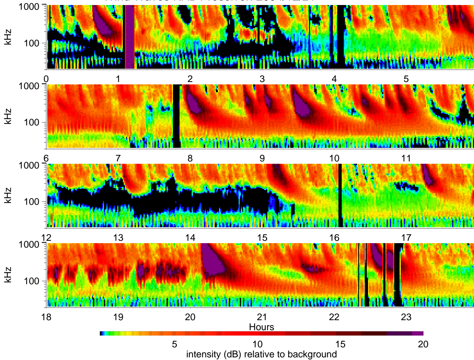
Wind Waves RAD1 receiver: 2004/12/21
