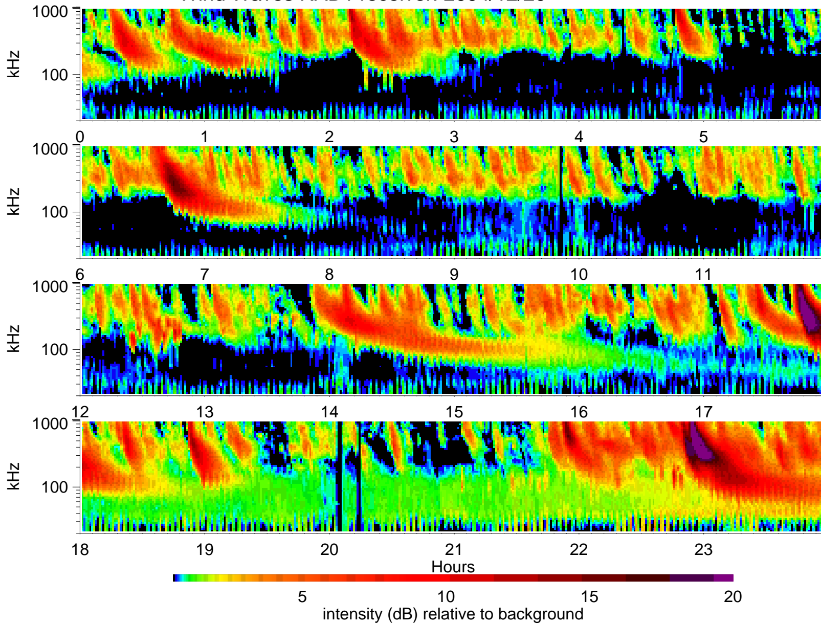
Wind Waves RAD1 receiver: 2004/12/20
