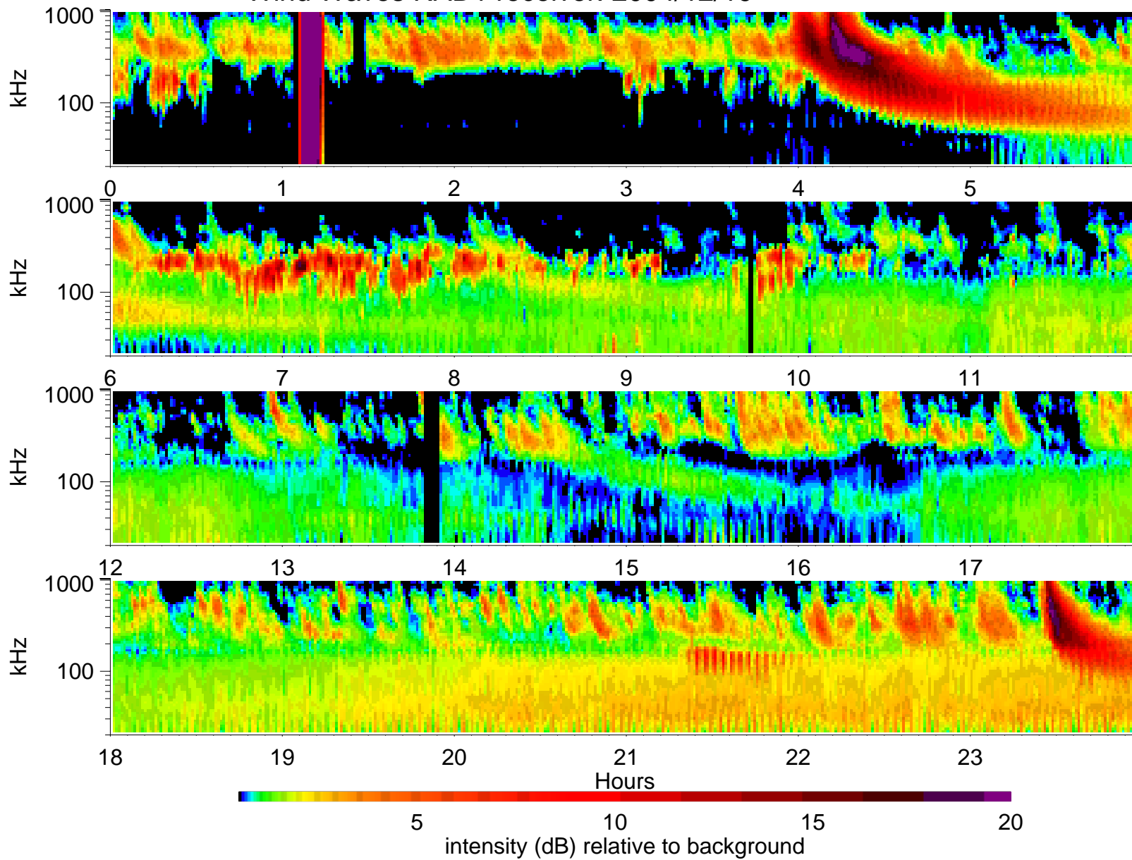
Wind Waves RAD1 receiver: 2004/12/19
