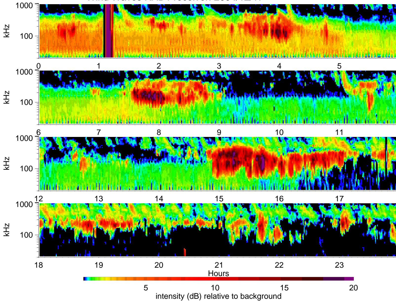
Wind Waves RAD1 receiver: 2004/12/17
