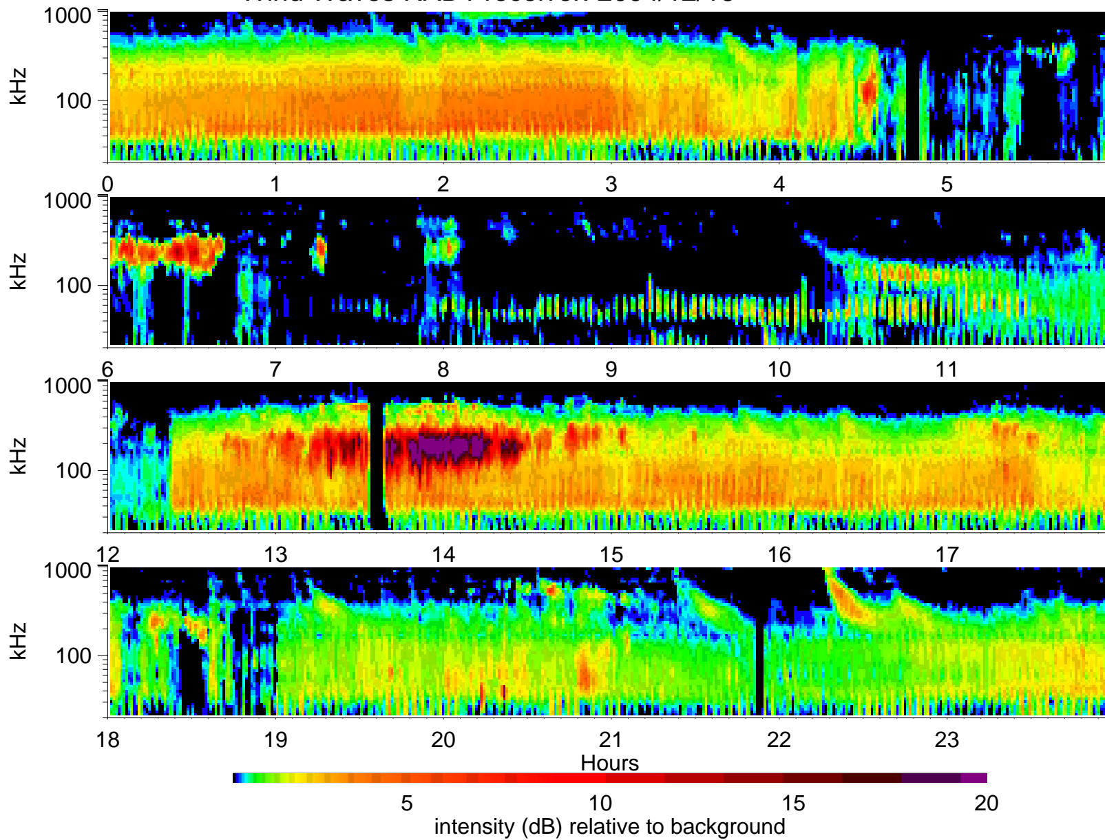
Wind Waves RAD1 receiver: 2004/12/16
