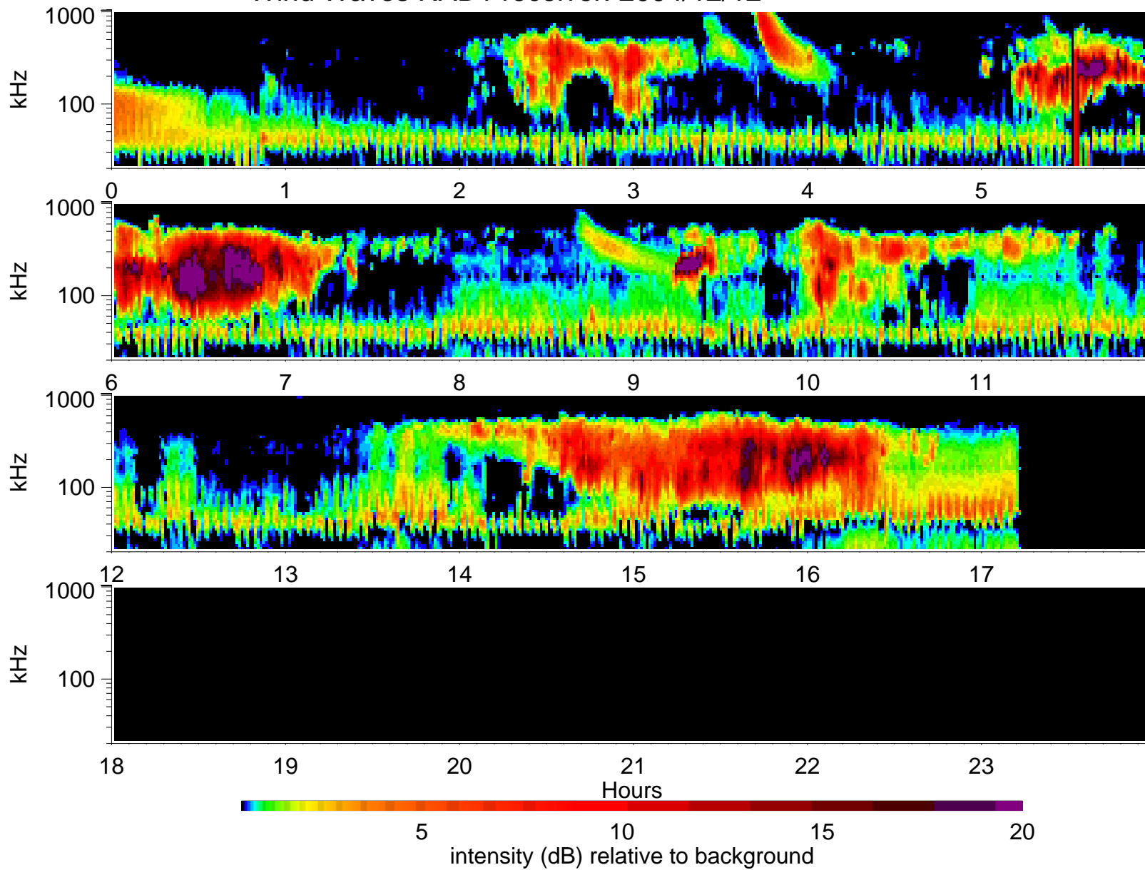
Wind Waves RAD1 receiver: 2004/12/12
