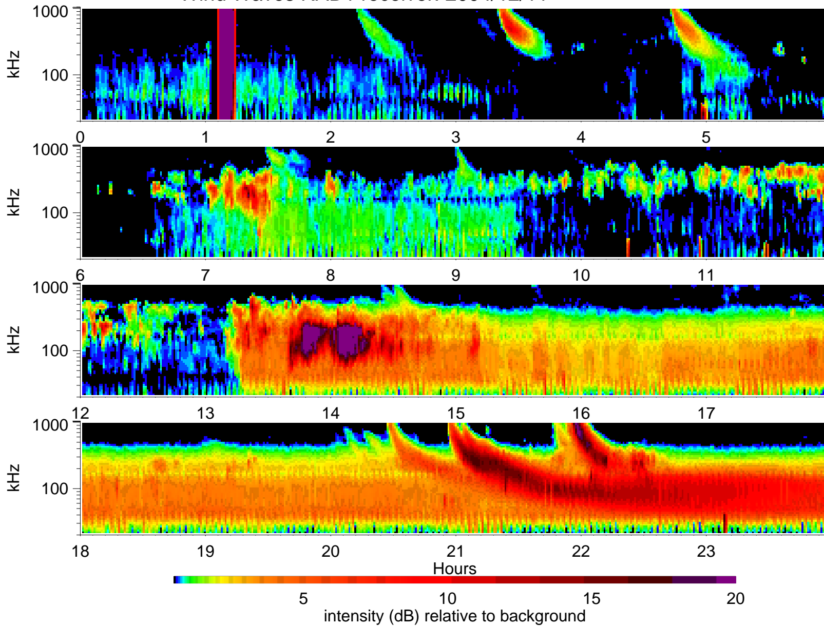
Wind Waves RAD1 receiver: 2004/12/11
