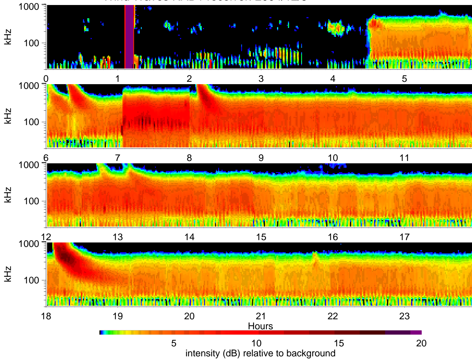
Wind Waves RAD1 receiver: 2004/12/5
