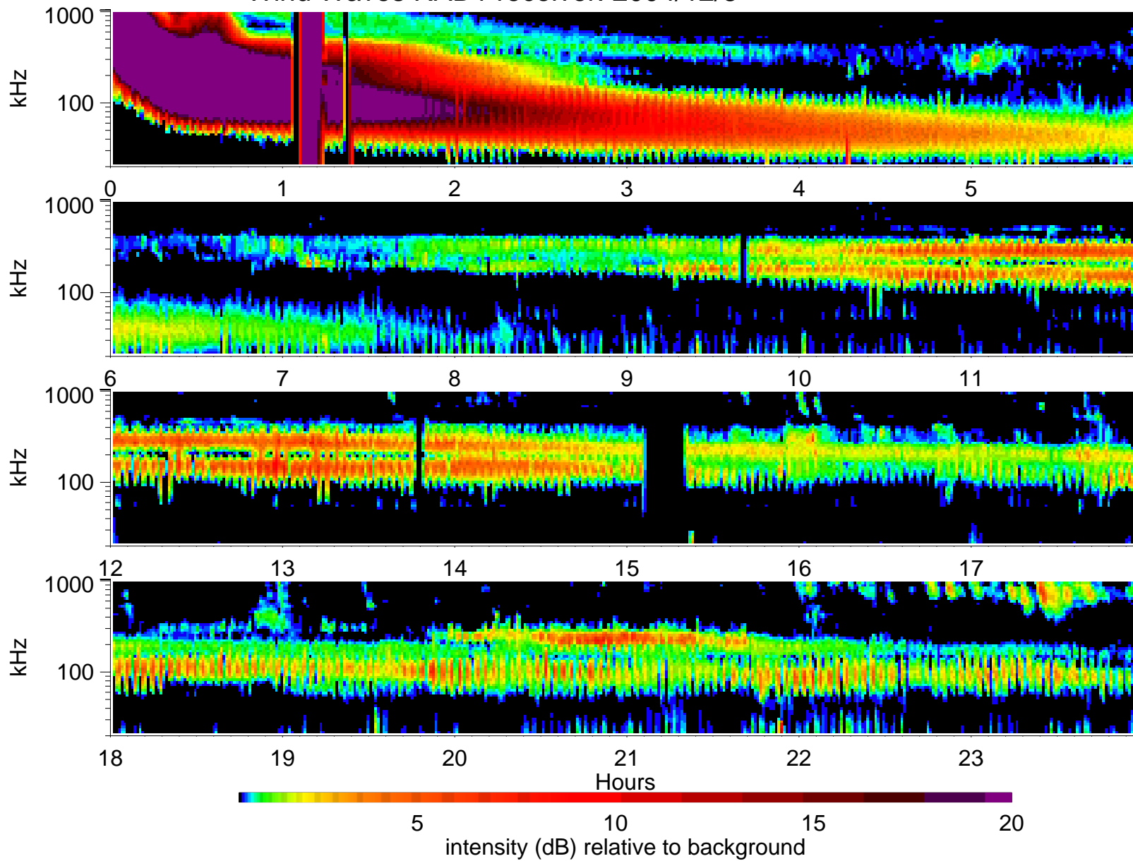
Wind Waves RAD1 receiver: 2004/12/3
