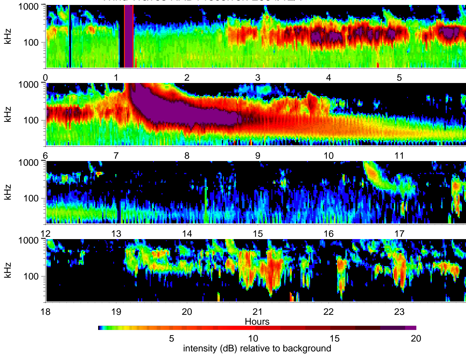
Wind Waves RAD1 receiver: 2004/12/1
