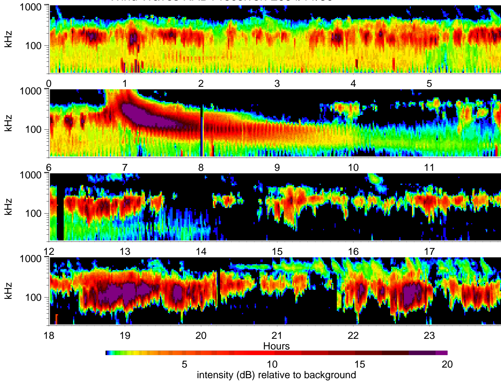
Wind Waves RAD1 receiver: 2004/11/30
