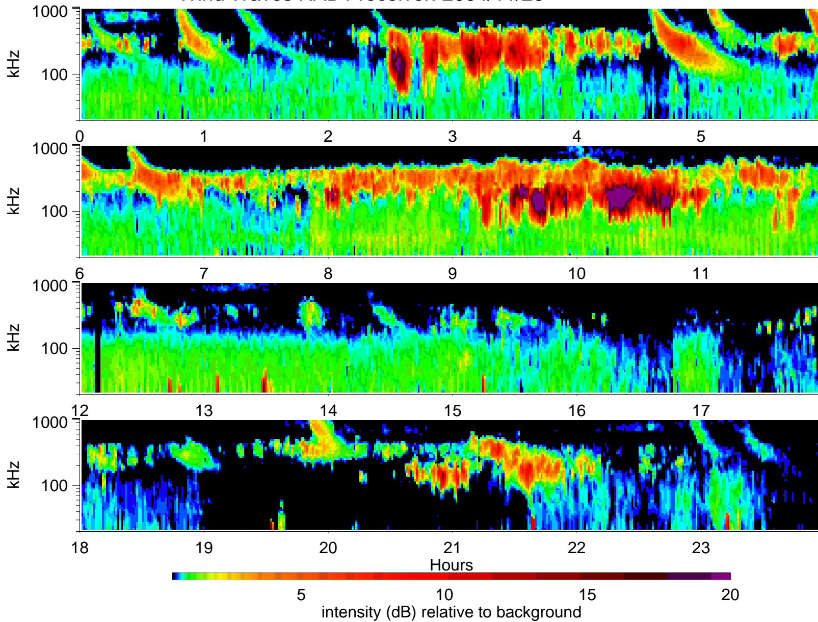
Wind Waves RAD1 receiver: 2004/11/26
