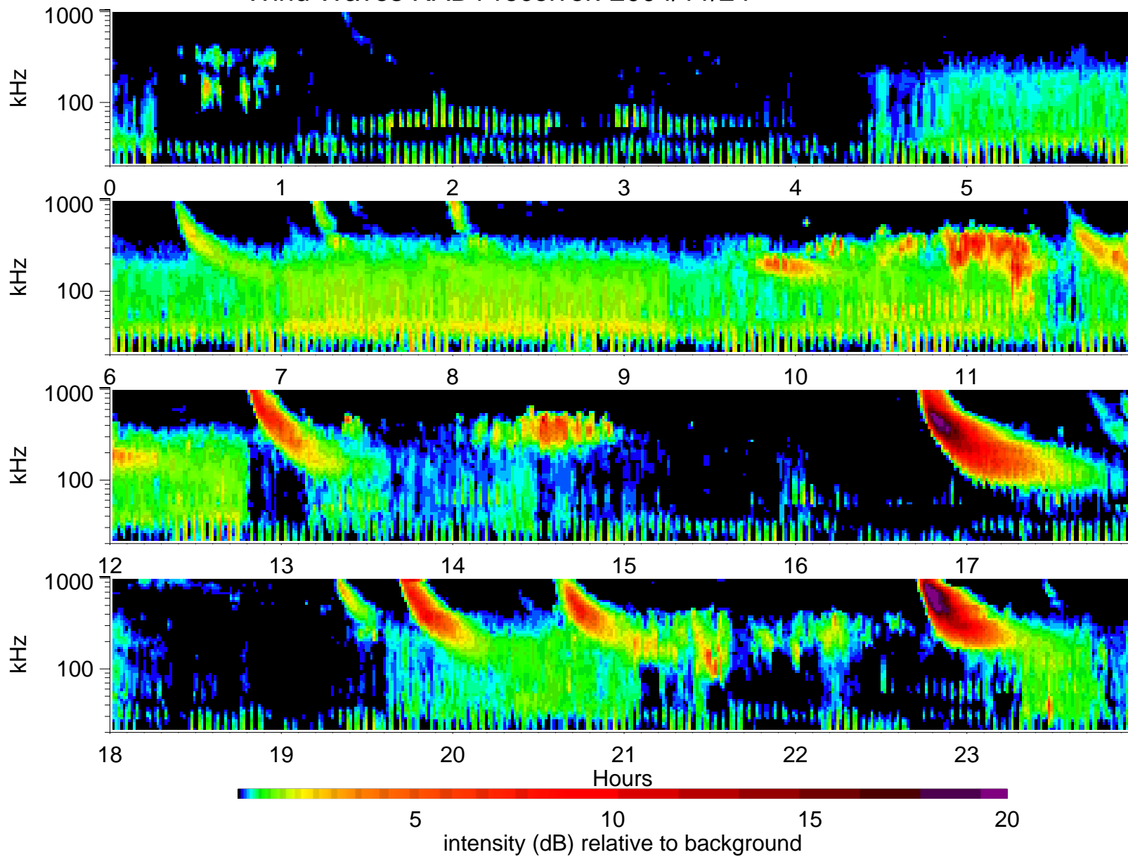
Wind Waves RAD1 receiver: 2004/11/24
