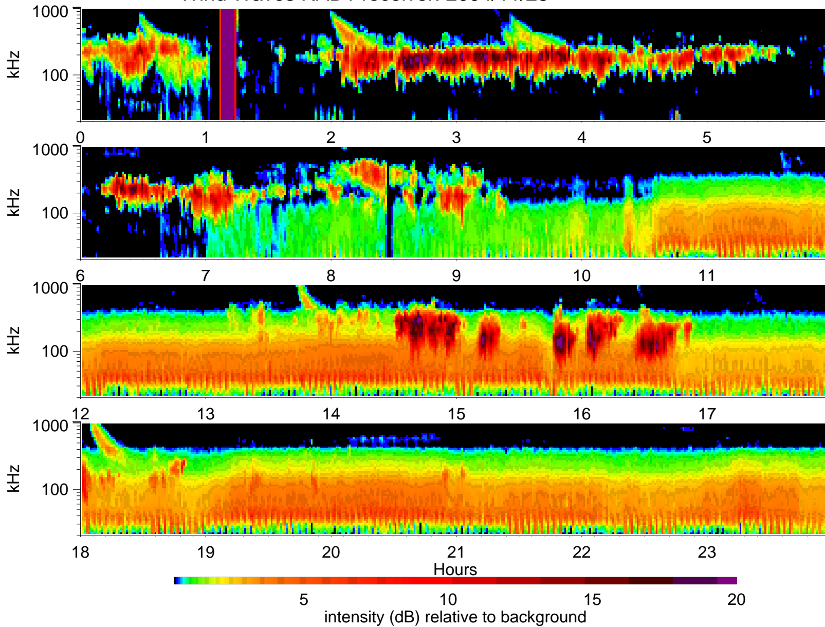
Wind Waves RAD1 receiver: 2004/11/23
