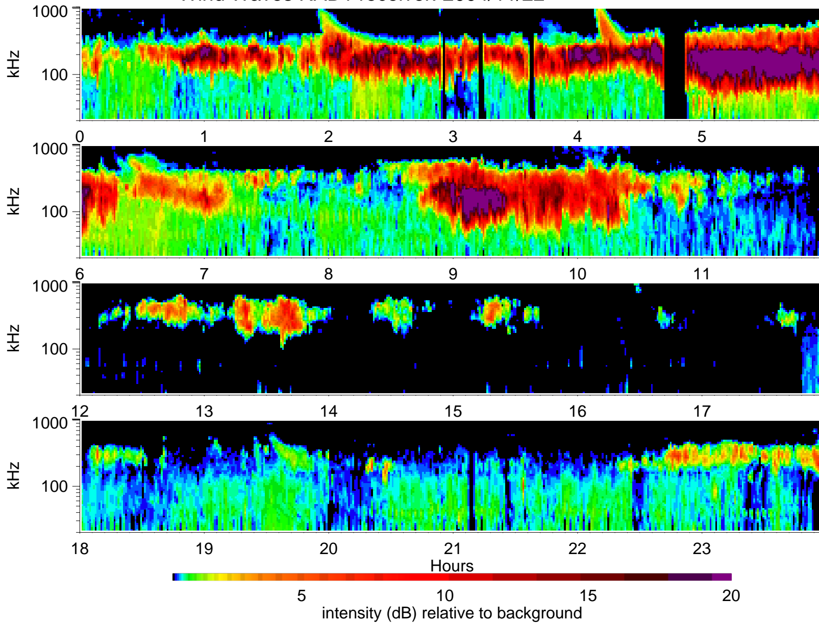
Wind Waves RAD1 receiver: 2004/11/22
