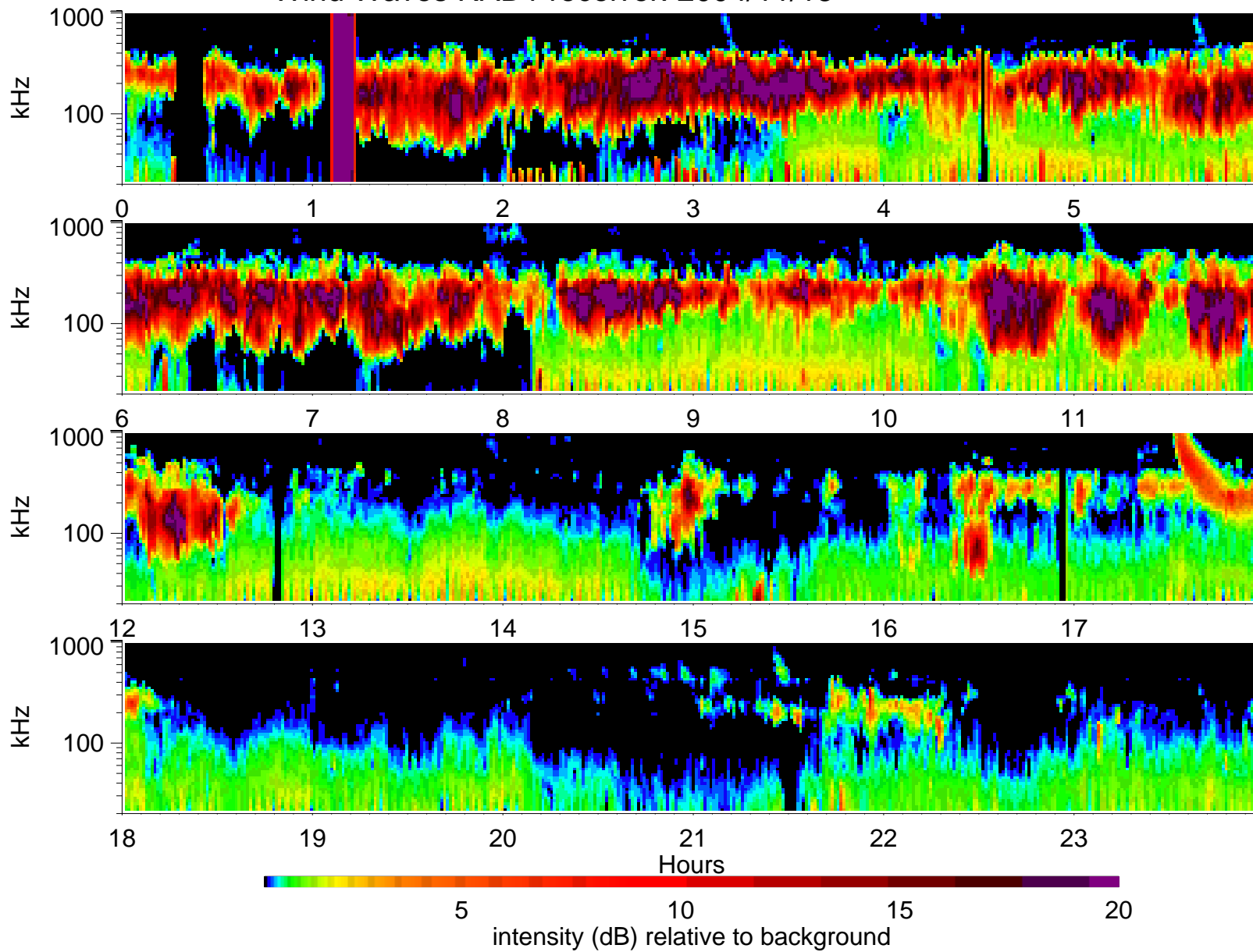
Wind Waves RAD1 receiver: 2004/11/13
