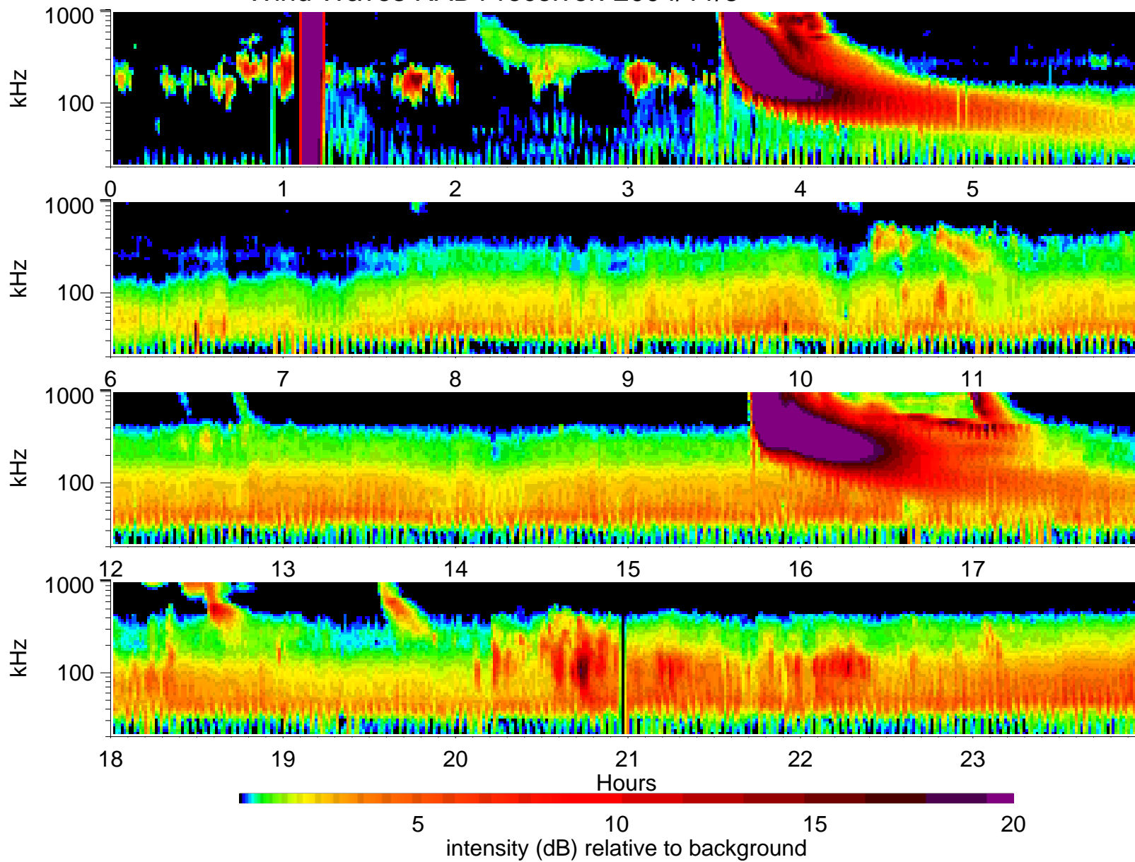
Wind Waves RAD1 receiver: 2004/11/3
