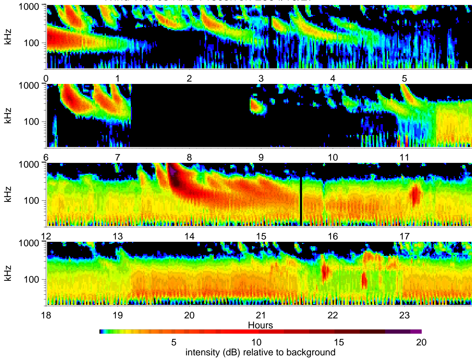
Wind Waves RAD1 receiver: 2004/10/27
