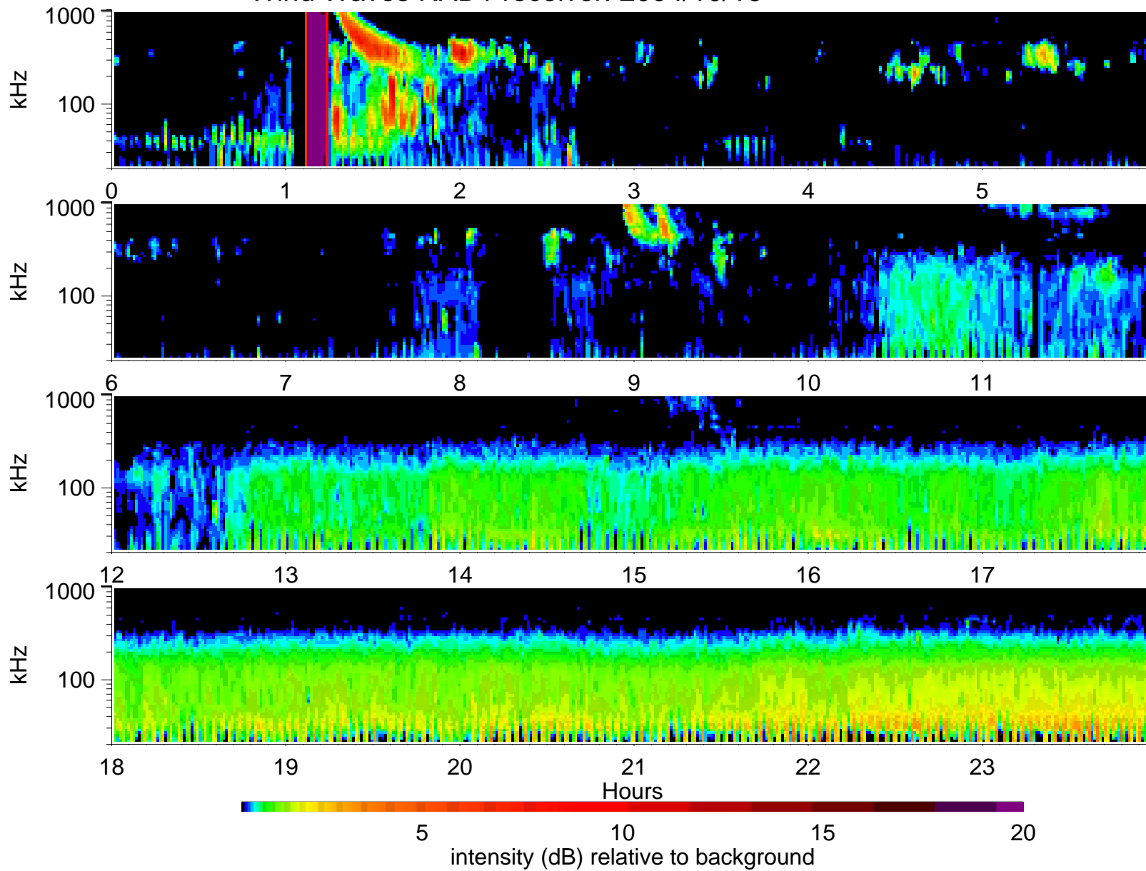
Wind Waves RAD1 receiver: 2004/10/16
