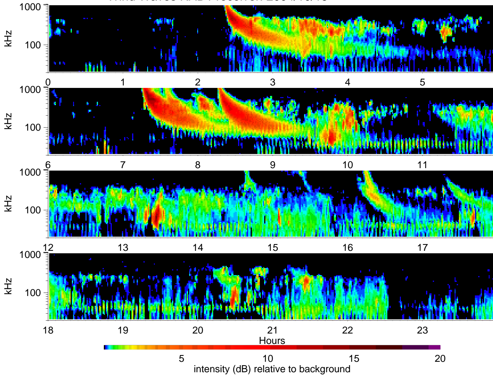
Wind Waves RAD1 receiver: 2004/10/15
