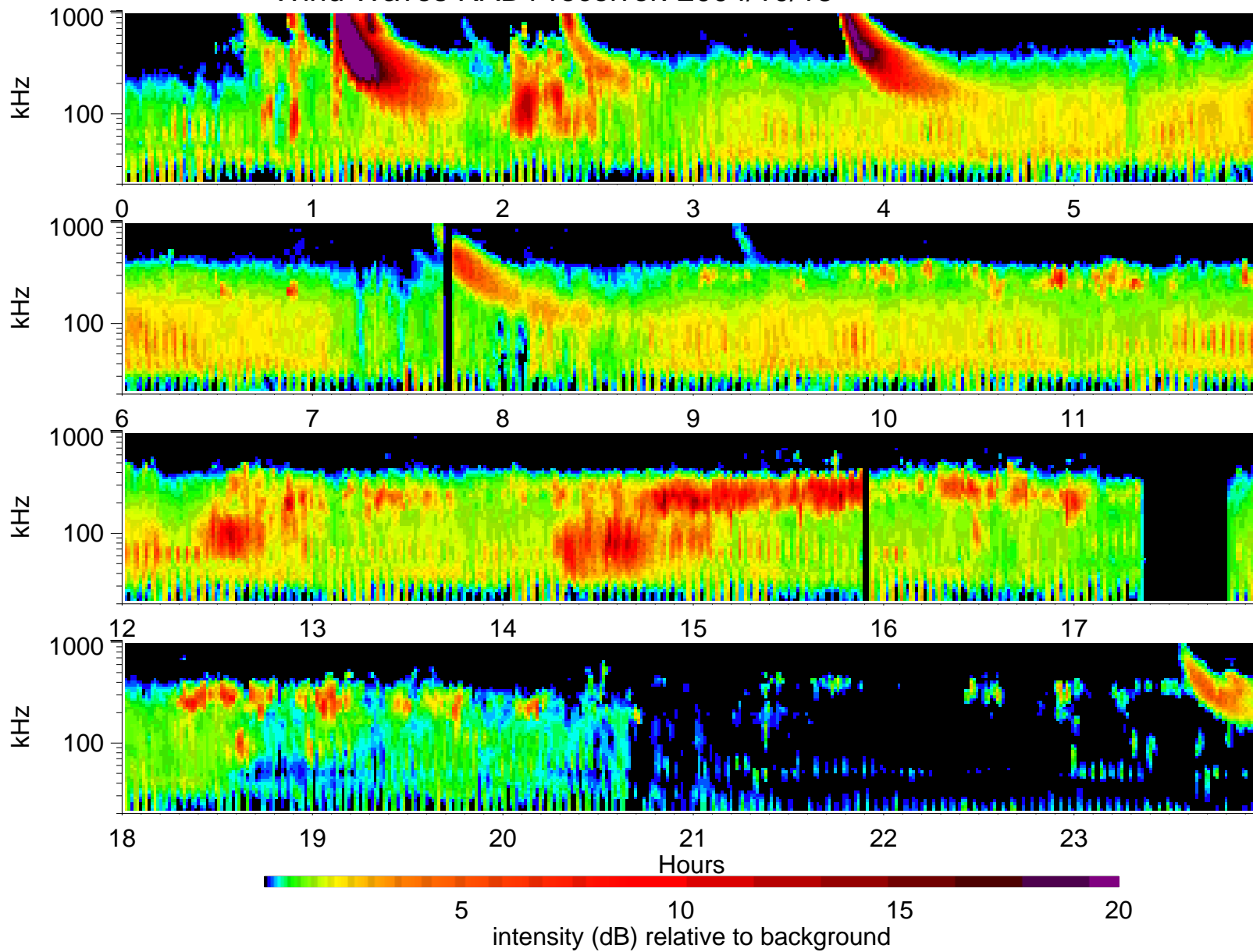
Wind Waves RAD1 receiver: 2004/10/13
