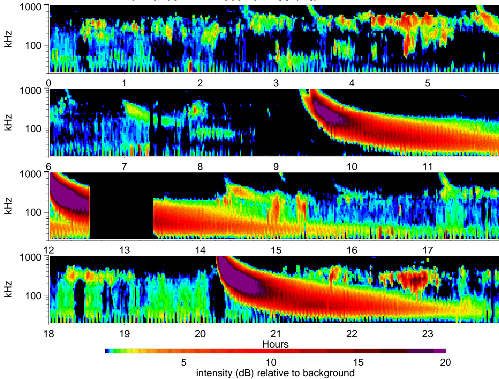
Wind Waves RAD1 receiver: 2004/10/11
