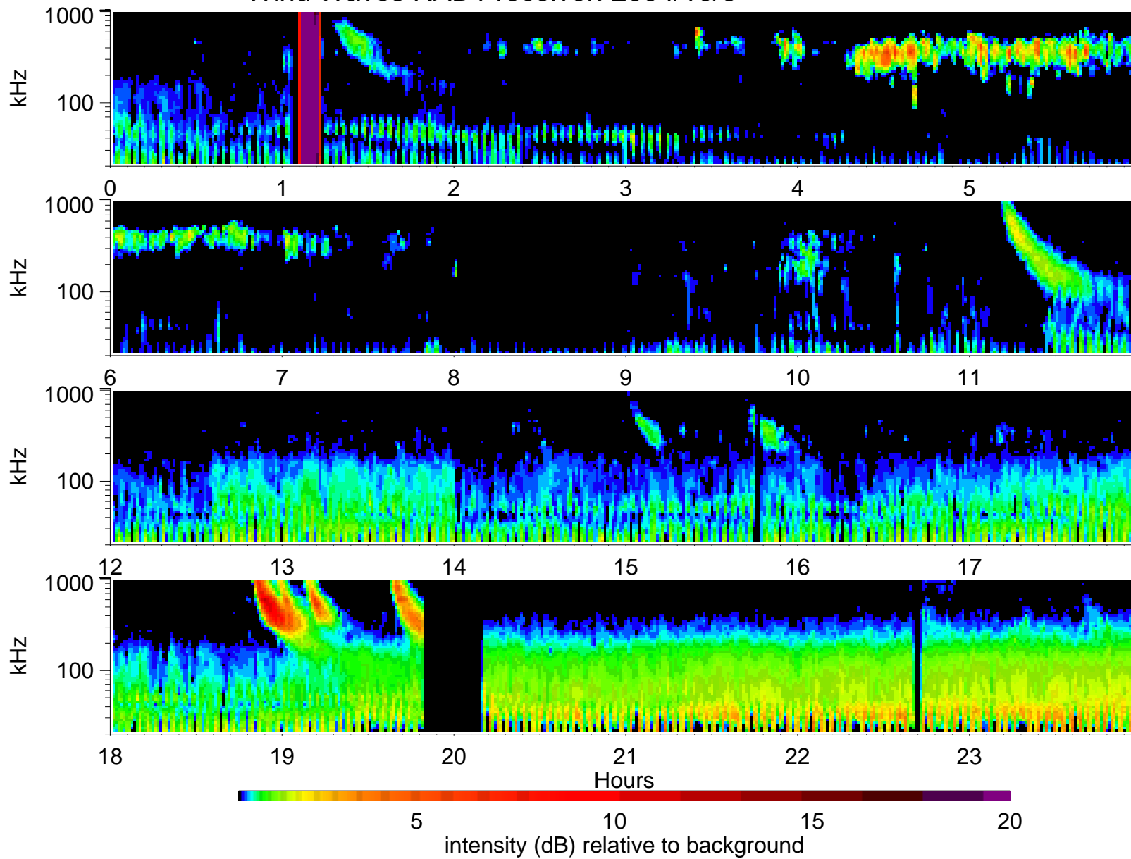
Wind Waves RAD1 receiver: 2004/10/6
