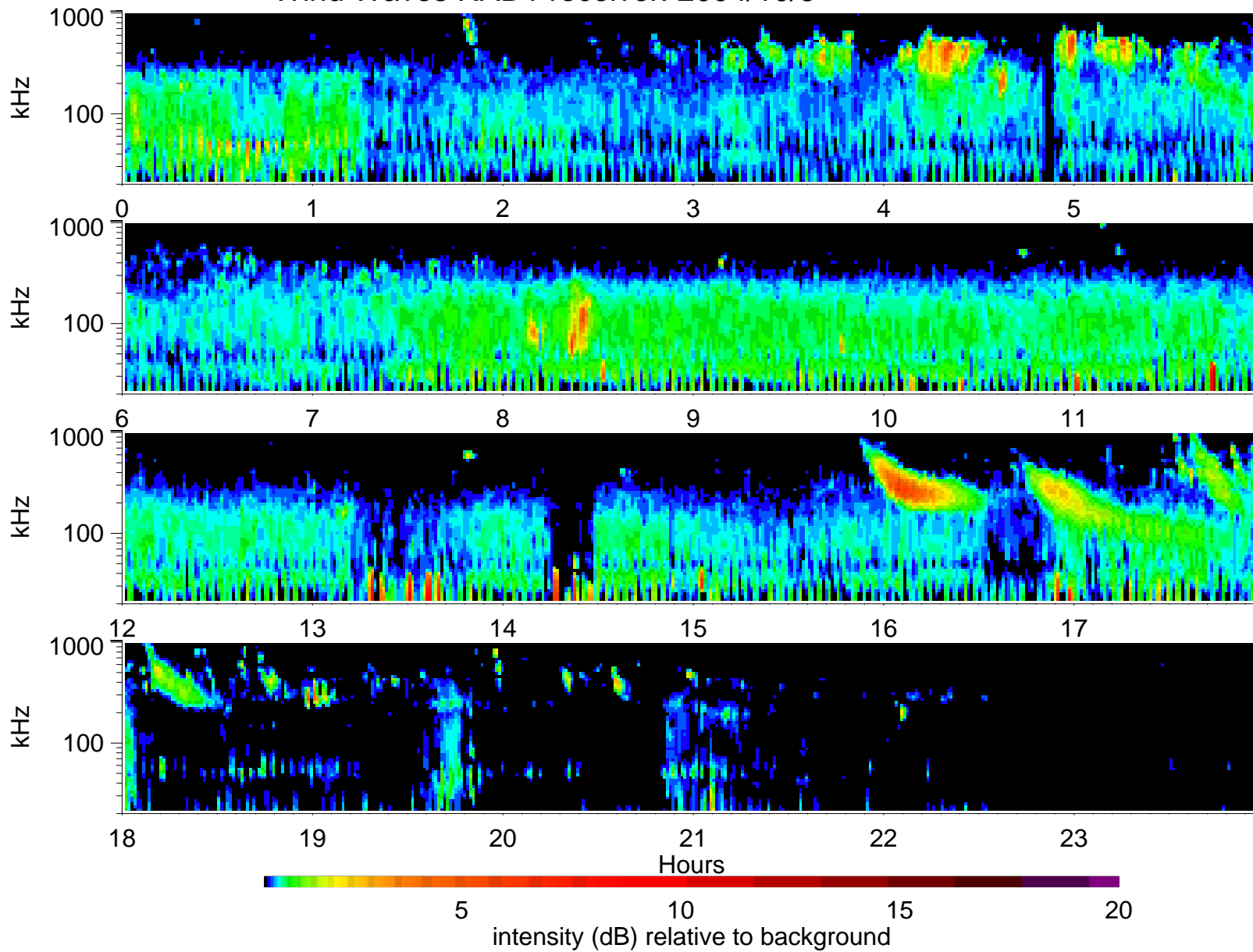
Wind Waves RAD1 receiver: 2004/10/5
