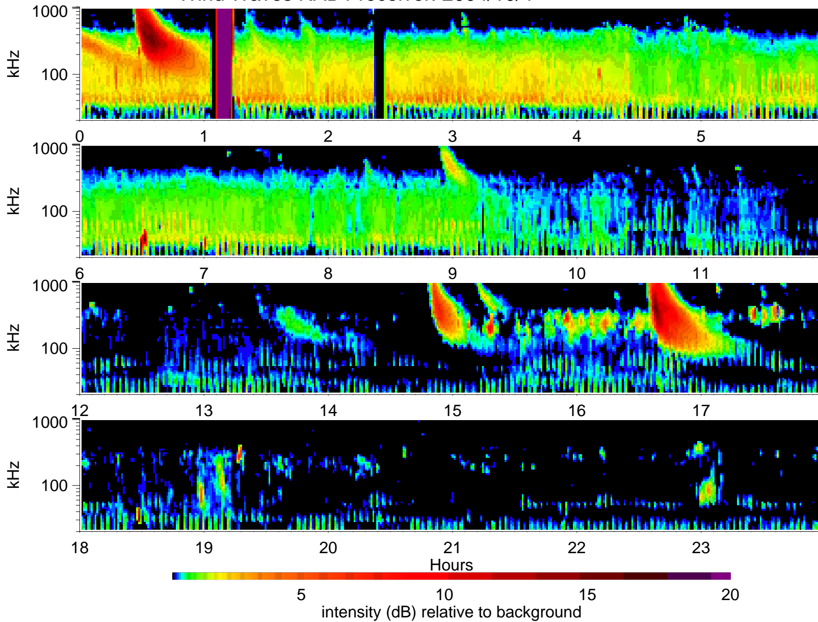
Wind Waves RAD1 receiver: 2004/10/4
