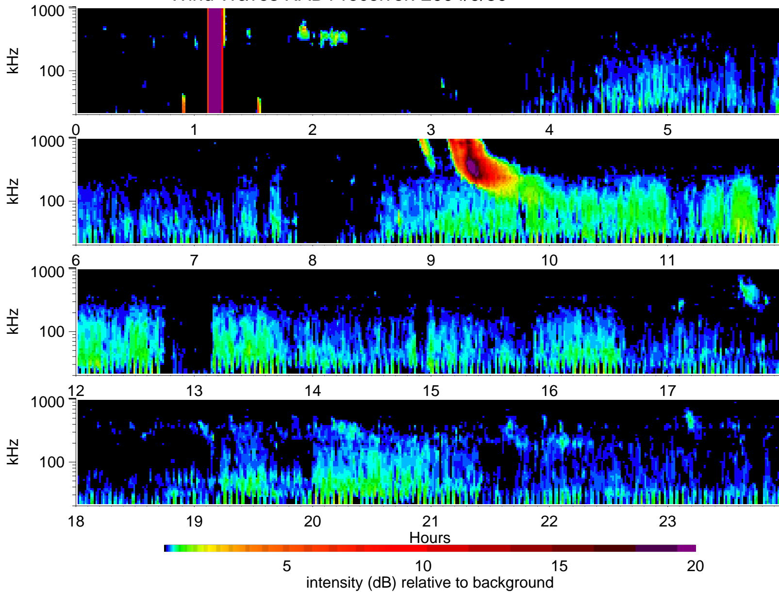
Wind Waves RAD1 receiver: 2004/9/30
