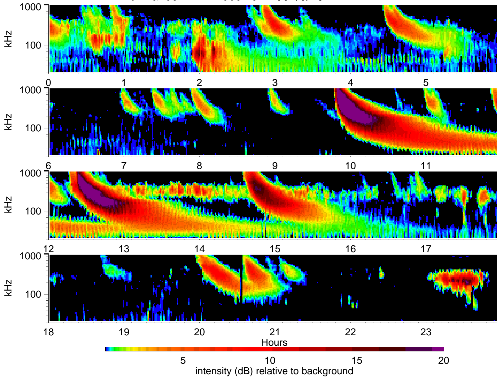
Wind Waves RAD1 receiver: 2004/9/23
