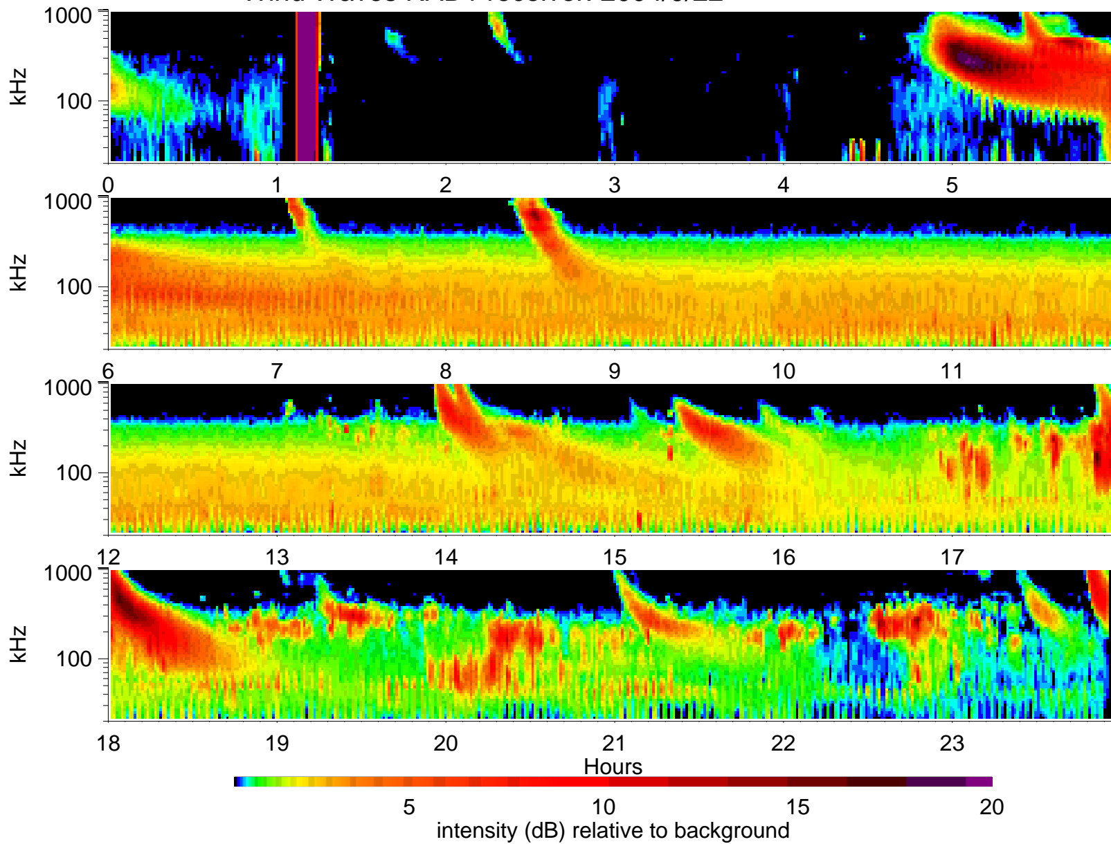
Wind Waves RAD1 receiver: 2004/9/22
