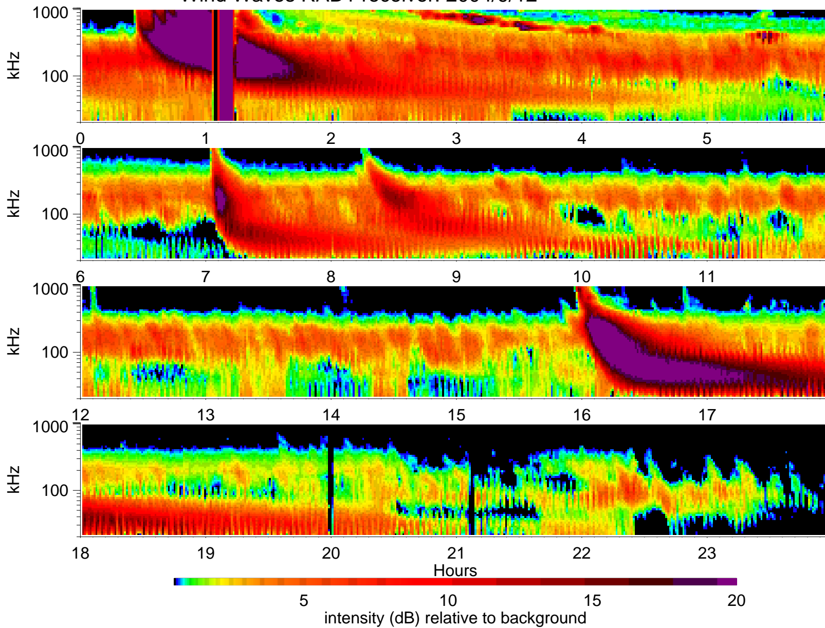
Wind Waves RAD1 receiver: 2004/9/12
