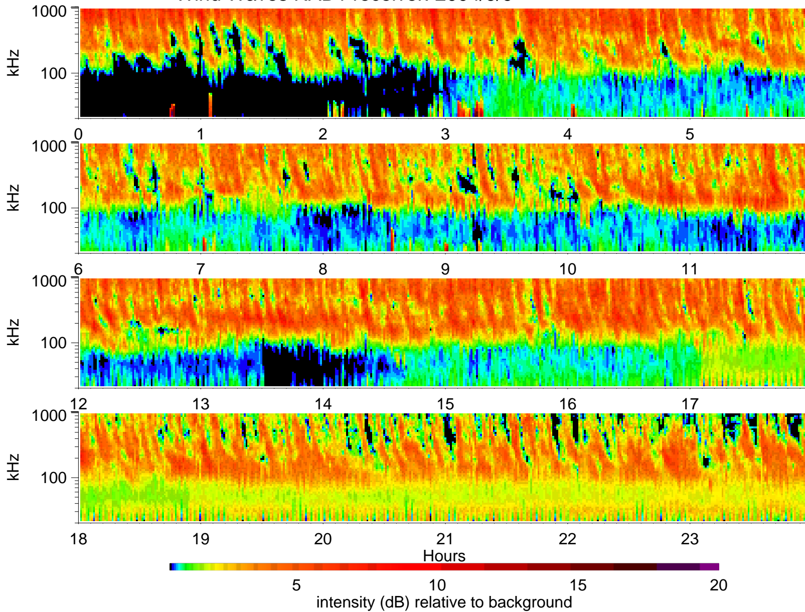
Wind Waves RAD1 receiver: 2004/9/9
