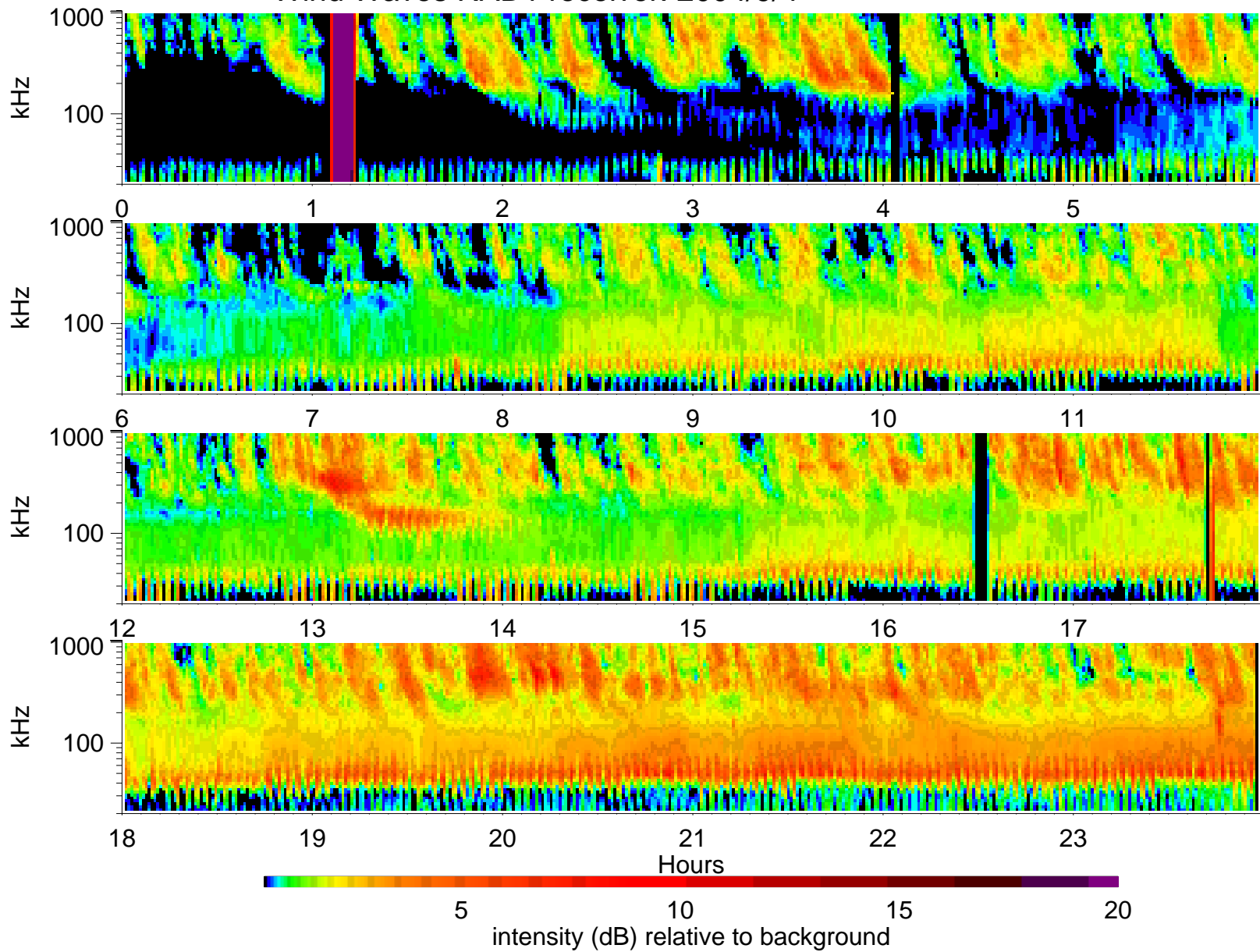
Wind Waves RAD1 receiver: 2004/9/4
