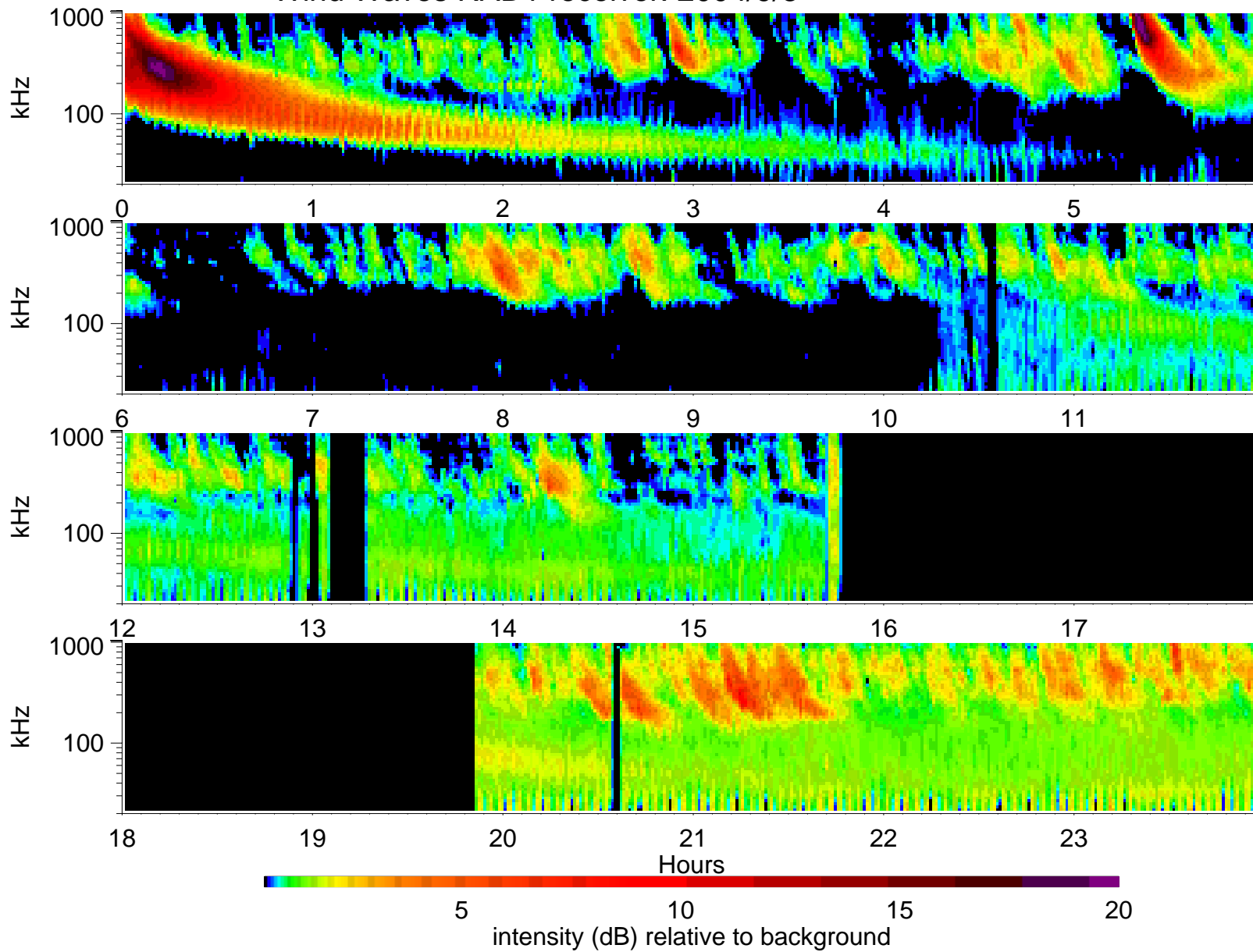
Wind Waves RAD1 receiver: 2004/9/3
