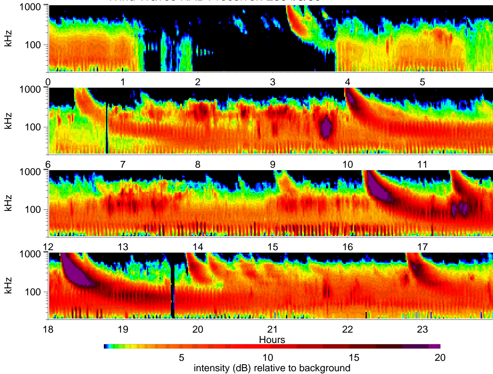
Wind Waves RAD1 receiver: 2004/8/30
