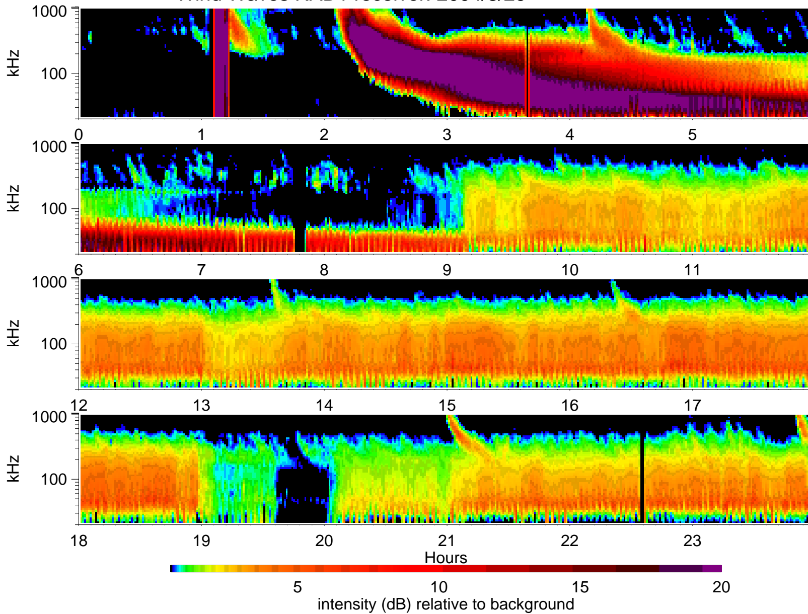
Wind Waves RAD1 receiver: 2004/8/29
